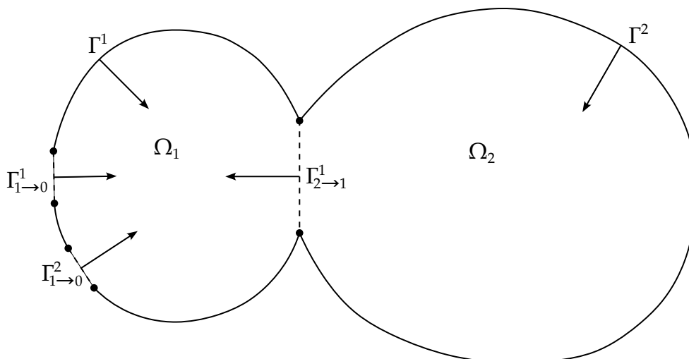
Figure 17-7. Two control volume with one sharing flow areas with the ambient environment. Control volume 1, \Omega_1 , has boundary \Gamma_1 . It shares two flow areas, \Gamma_{1 \rightarrow 0}^1 and \Gamma_{1 \rightarrow 0}^2 , with the ambient environment, and one flow area \Gamma_{2 \rightarrow 1}^1 , with control volume 2, \Omega_2 . \Omega_2 has boundary \Gamma_2 and only shares flow areas with \Omega_1 . See Remarks 1, 2, and 5 .
