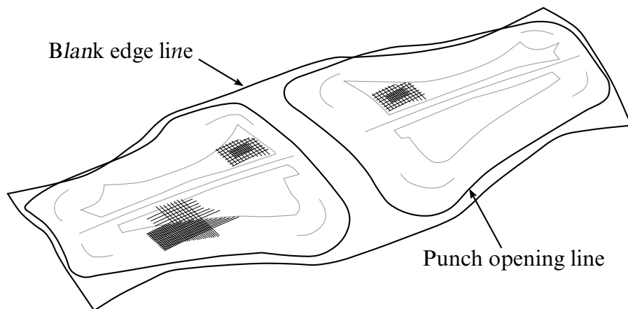
Figure 17-28. The fender outer (draw complete) in wireframe mode.
