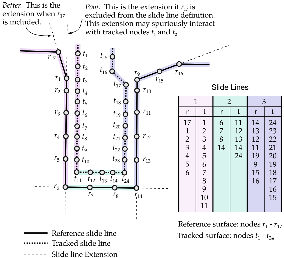
Figure 11-36. Slide line Example. Note: (1) as recommended, for 90° angles each facet is assigned a distinct slide line; (2) the reference slide line is more coarsely meshed; (3) the tracked slide line is to the left of the reference (following the node ordering, see inset table); (4) as shown for tracked nodes 1 and 2 it is important the slide line extension does not spuriously come into contact.
