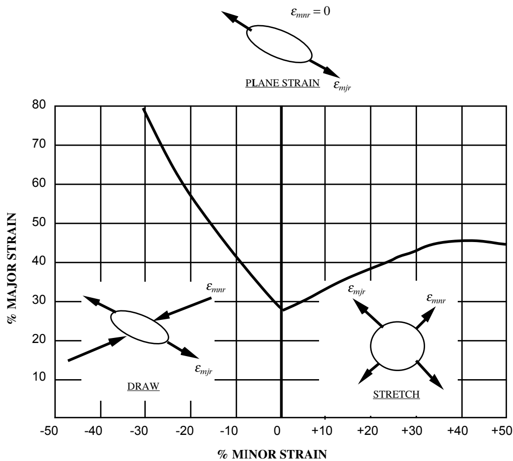
Figure 17-19. Flow limit diagram.
