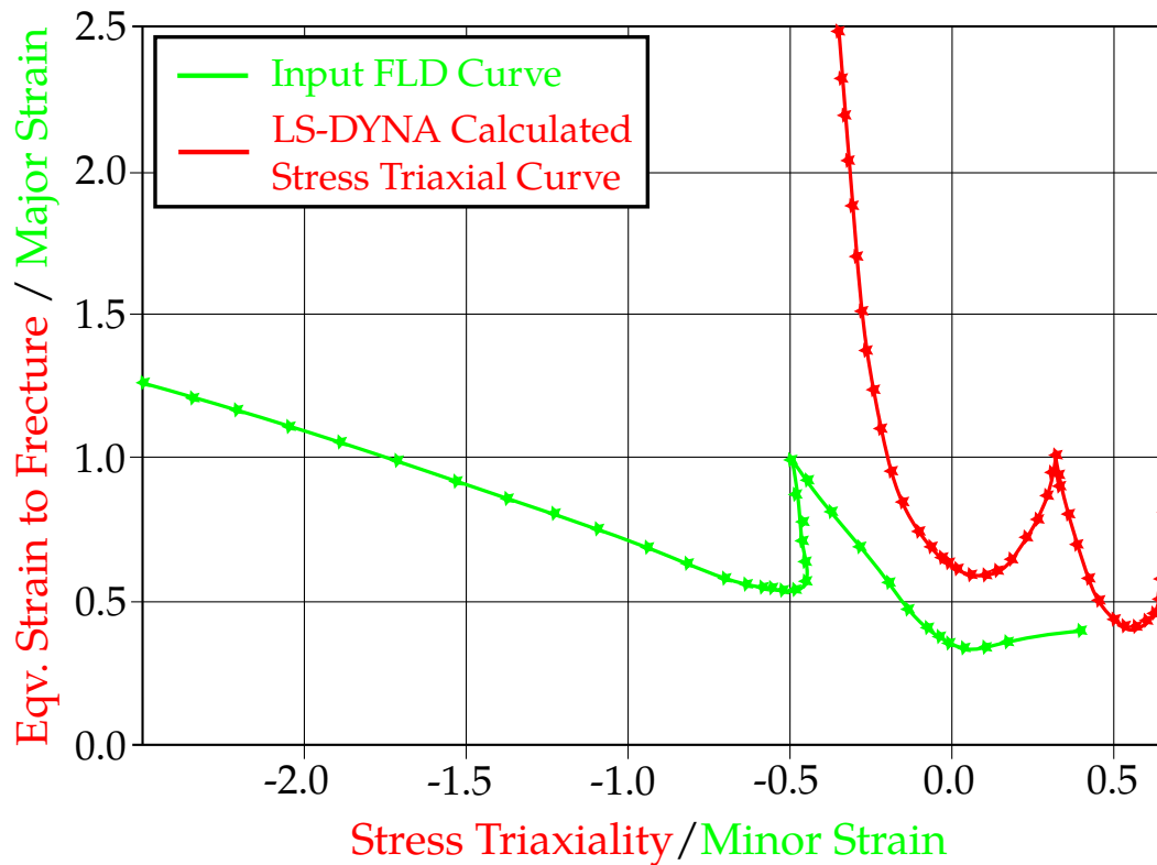
Figure 17-24. LS-DYNA calculated stress triaxial curve from FLD curve [1].
