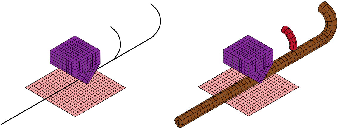
Figure 17-6. Example of initial beam geometry and resulting solid/beam geometry
