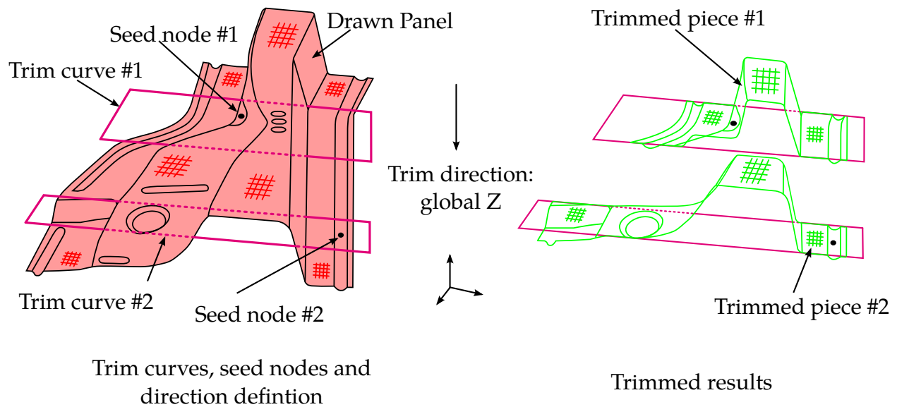
Figure 17-36. An example of 2D trimming of sandwiched part (laminates) from 2005 NUMISHEET benchmark - cross member.
