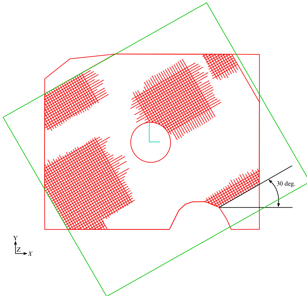
Figure 17-45. A rectangular blank mesh is generated in an angle (ANGLEX = 30) and trimmed into a developed blank shape, with an inner cutout defined by innerhole.iges and outline defined by outlines.iges . Note the blank mesh orientation is always parallel to the rectangular blank boundary.
