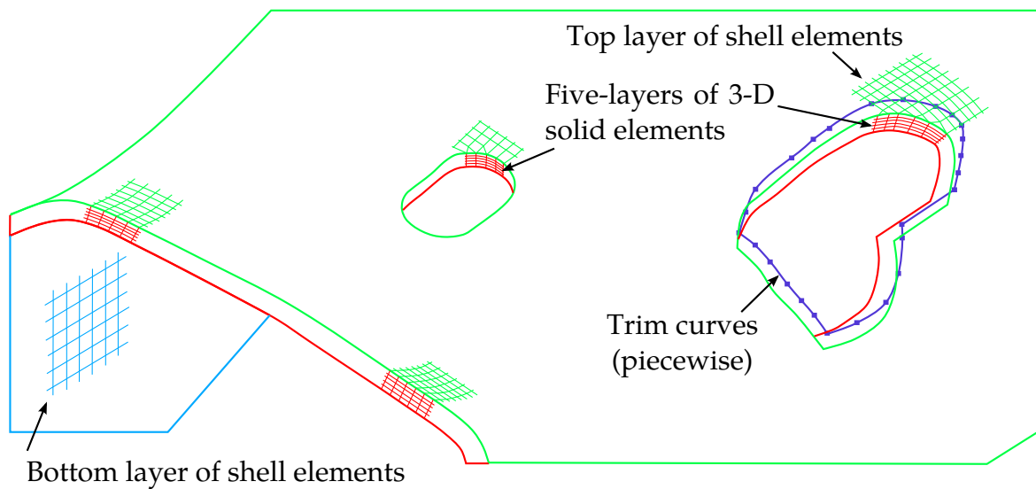
Figure 17-33. 3D trimming of laminates (a core of multiple-layers of solid elements with top and bottom layers of shell elements) using *DEFINE_CURVE_TRIM_3D. Note that shell elements must share the same nodes with the solid elements at the top and bottom layer.
