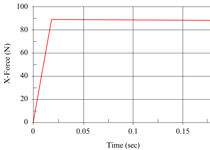
Figure 17-51. Pulling force (frictional force) from RCFORC file.
