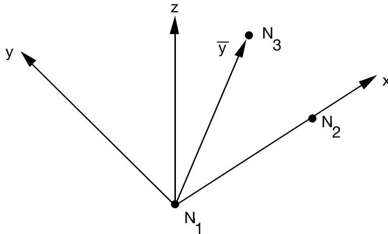
Figure 17-8. Definition of local coordinate system using three nodes when the node N_2 lies along the x -axis.
