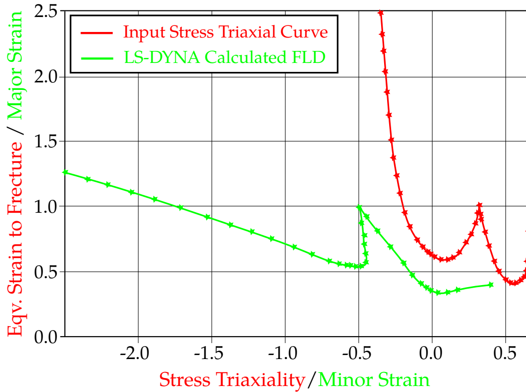
Figure 17-22. LS-DYNA calculated FLD from input stress triaxial curve [1].
