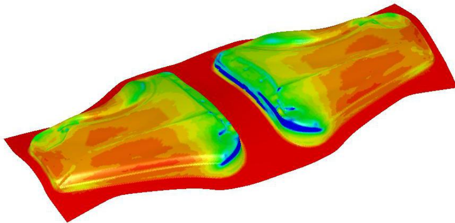
Figure 17-29. The fender outer - thickness/thinning plot on the drawn panel.
