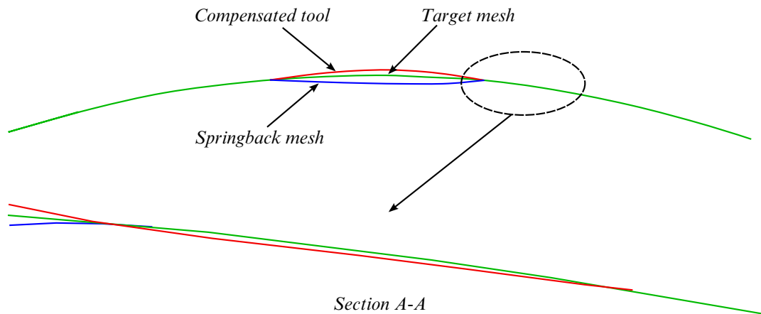
Figure 17-17. Local compensation details.
