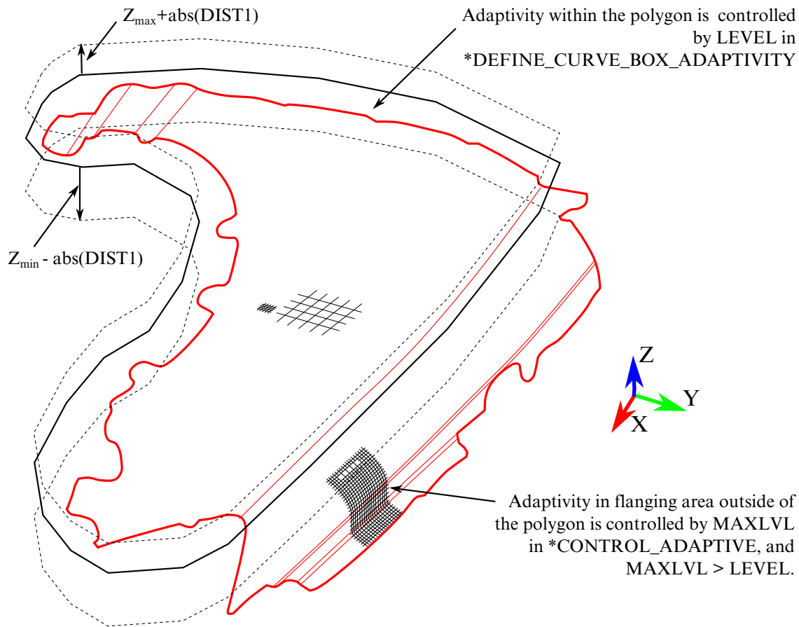
Figure 17-14. Defining an adaptive polygon box
