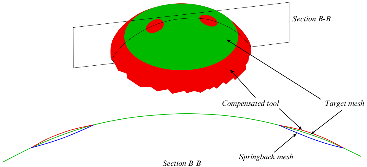
Figure 17-18. Multi-region local compensation.
