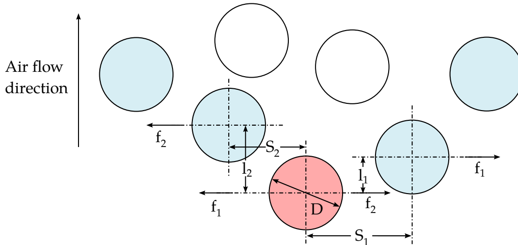
Figure 17-38. Illustration of perpendicular drag force in the lead particles for DFLAG = 2 and 3. In this schematic, the red particle interacts with both of its neighbors.
