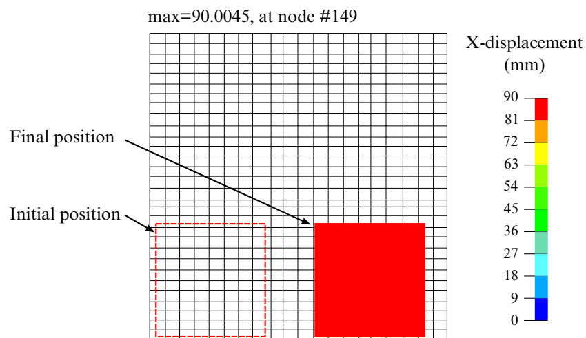
Figure 17-49. Initial and final position of the blank.
