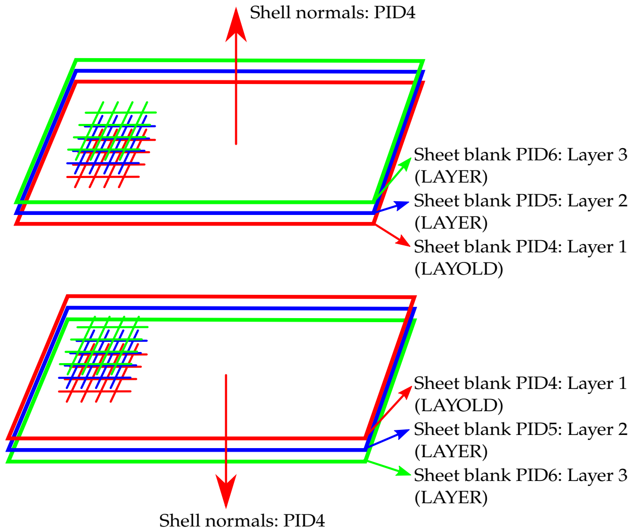
Figure 17-58. Defining the variables LAYER and LAYOLD.
