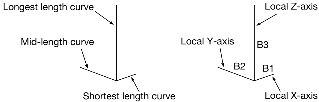
Figure 17-11. Input curves (left). The generated local coordinate system is written to the d3plot file as a part consisting of three beams (right).
