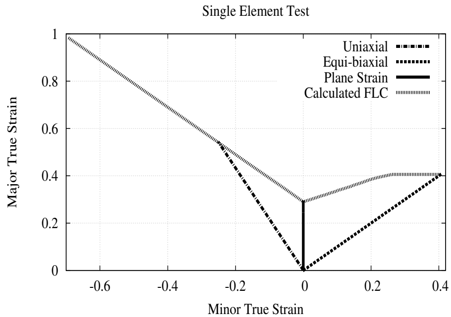
Figure 17-21. Validation of the FLC defined by this keyword
