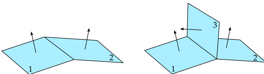
Figure 17-42. Bending in fabric, intended use of *DEFINE_FABRIC_ASSEMBLIES. The numbers indicate the parts the elements belong to.
