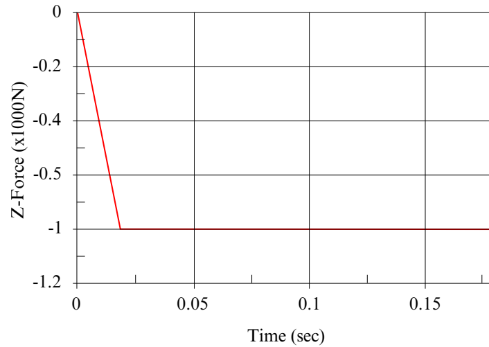
Figure 17-50. Normal force from RCFORC file.
