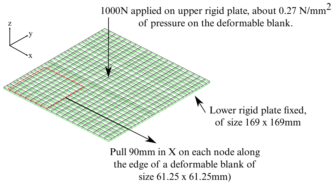
Figure 17-48. Boundary and loading conditions of a small test model.
