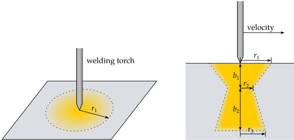
Figure 5-16. Heat source distribution geometry for IFORM = 3
