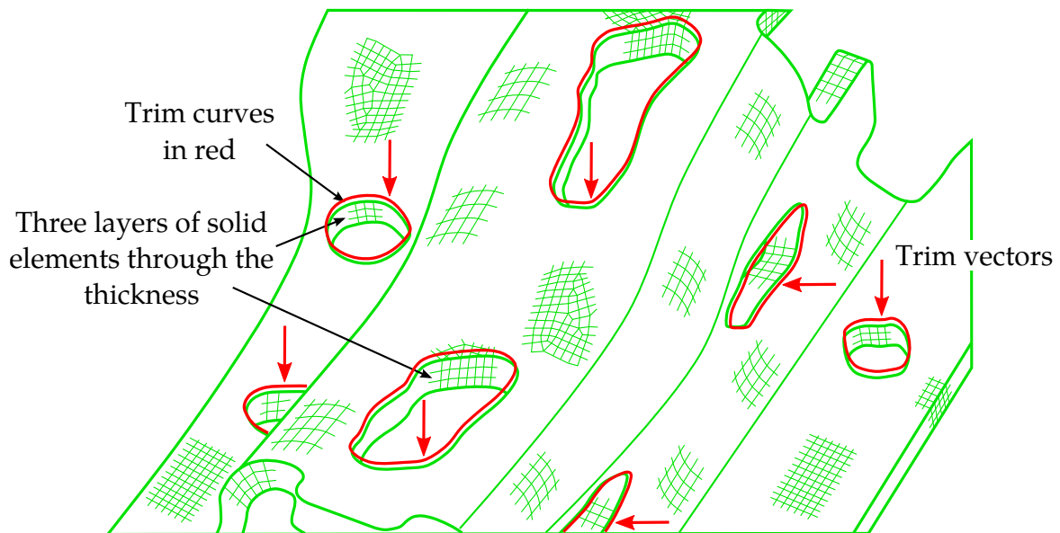
Figure 17-32. 2D trimming of solids using *DEFINE_CURVE_TRIM_2D
