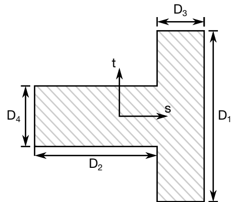
Figure 41-14. SECTION_14 \Rightarrow T-Shape 2
