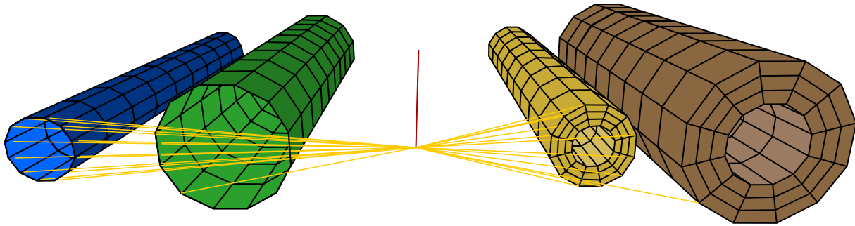
Figure 17-59. Automatically generated tubes using TYPE = 1, -1, 0, 2, and -2, from left to right. The beam tube ends are connected with *CONSTRAINED_NODAL_RIGID_BODY, which applies differently to the generated shell/solid tubes, depending on the sign of TYPE.
