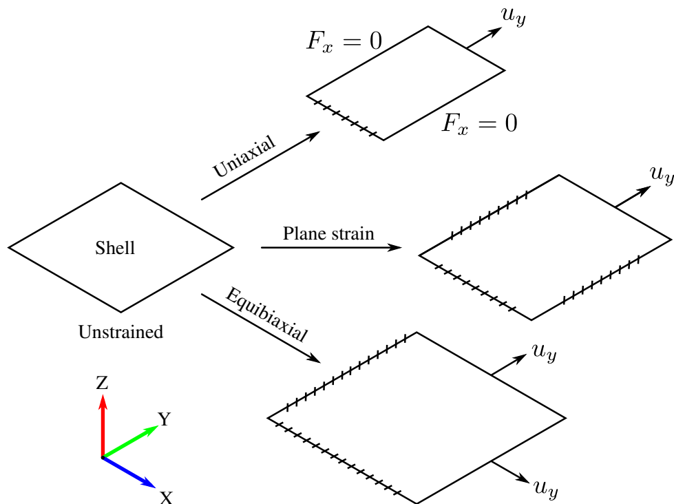
Figure 17-20. A single shell strained in three different strain paths
