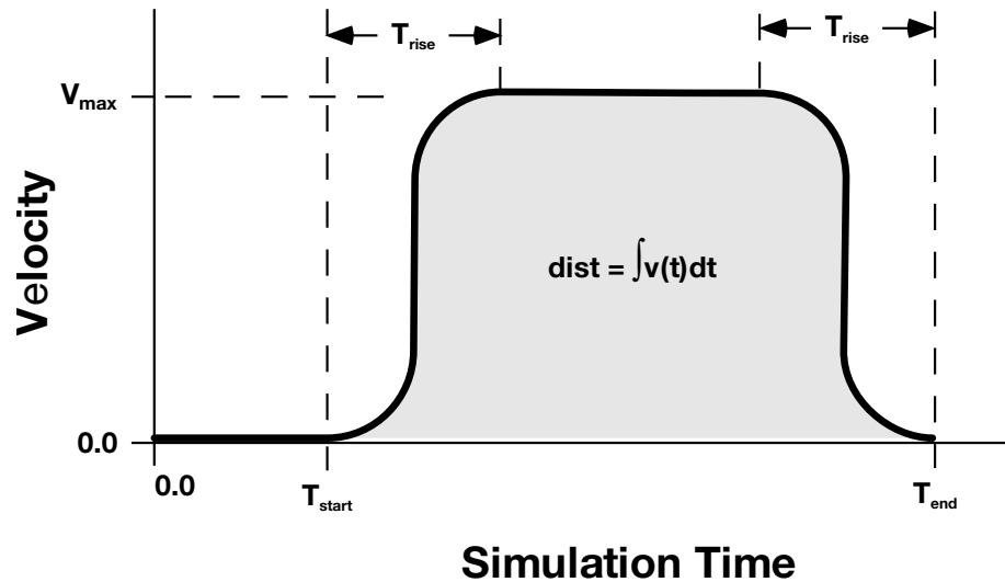
Figure 17-23. Smooth curve created automatically using *DEFINE_CURVE_SMOOTH. This shape is commonly used to control velocity of tools in metal forming applications as shown in this figure but can also be used for other applications in place of any standard load curve.
