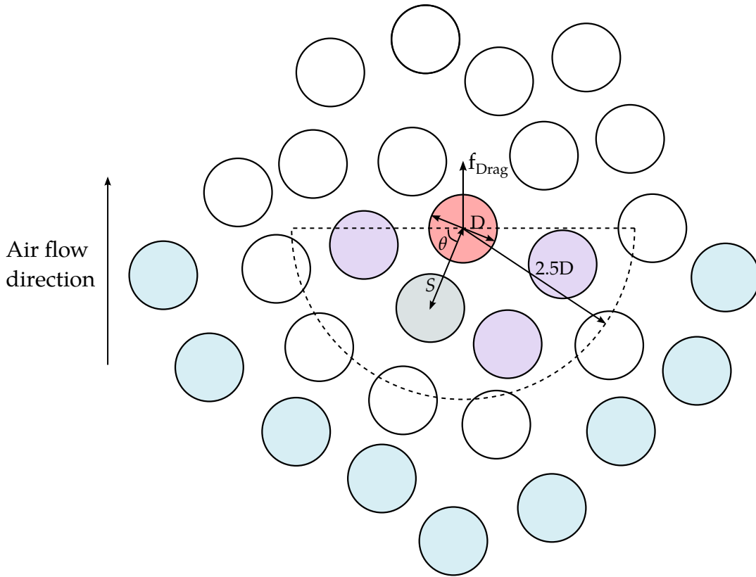
Figure 17-37. Schematic of how neighboring particles affect the drag treatment for DFLAG = 2 and 3. In this schematic the particles in blue are the leading particles that move at supersonic speed. We have developed two different methods for how the coefficient of drag is influenced by neighboring particles for particles that are not leading particles. In both methods, LS-DYNA checks for particles in the hemisphere in front of a given particle. In this schematic, the given particle is in red. The neighboring particles in the hemisphere are purple and grey. For DFLAG = 2, the grey particle is the closest neighbor of the red particle.
