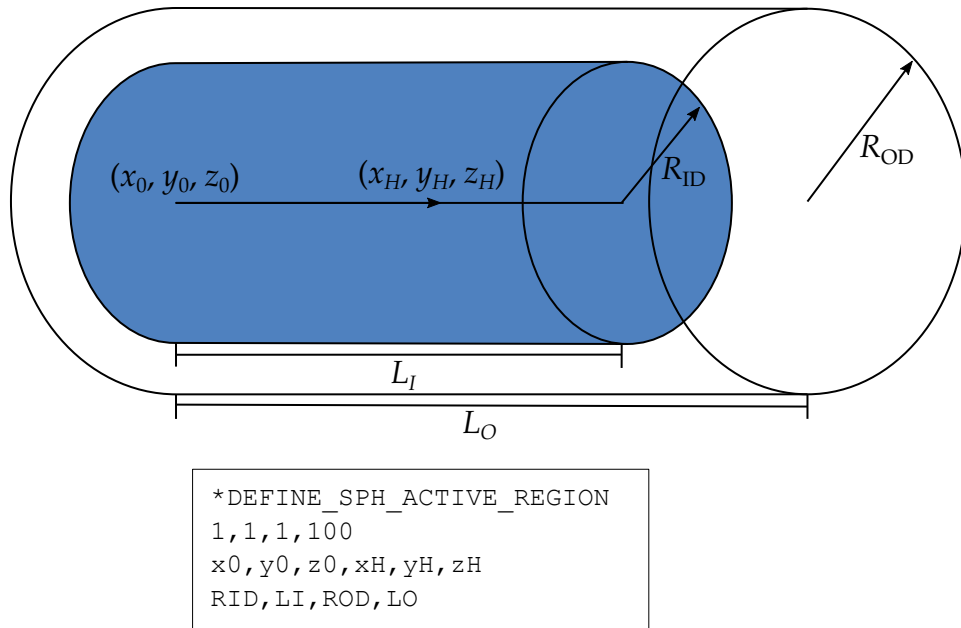
Figure 17-60. Example DEFINE_SPH_ACTIVE_REGION
