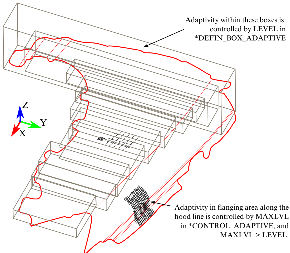
Figure 17-15. Defining adaptive boxes
