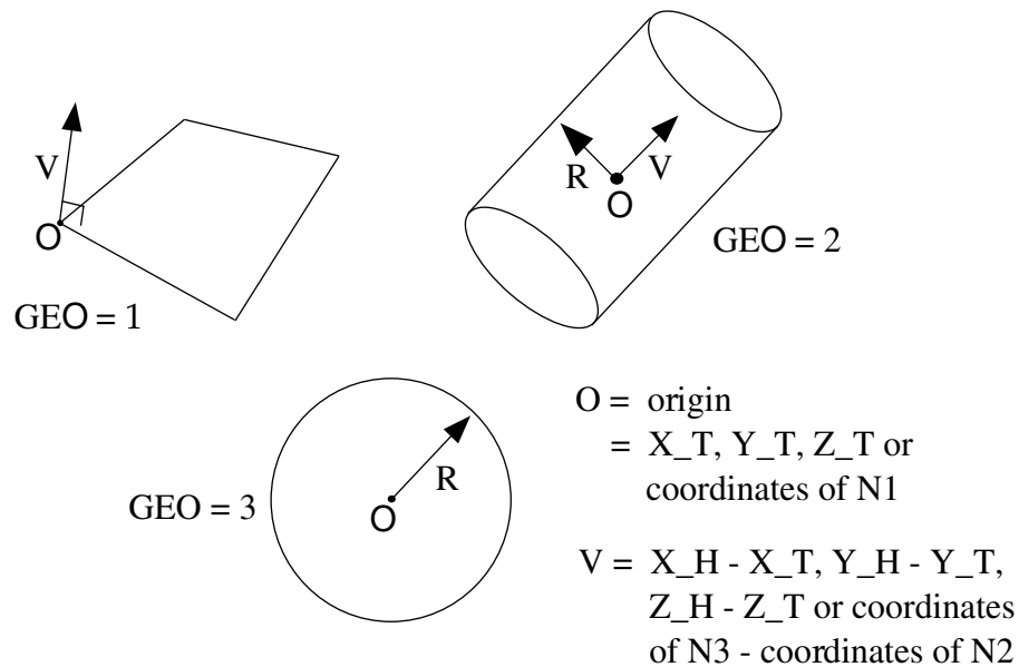
Figure 17-39. Geometry types.
