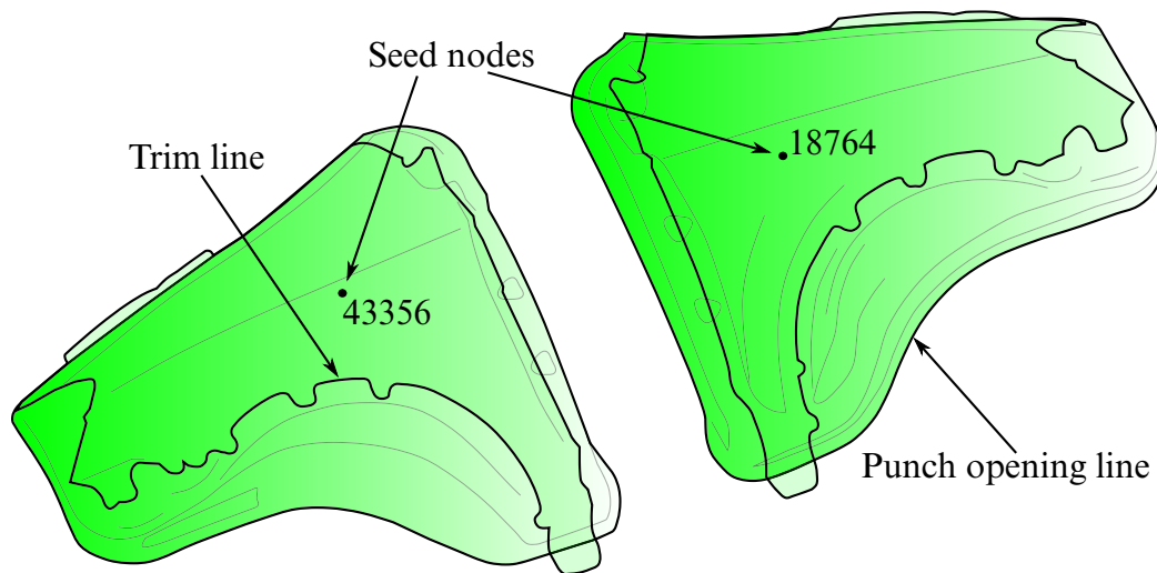
Figure 17-27. Trimming of a double-attached part (NUMISHEET2002 Fender Outer).
