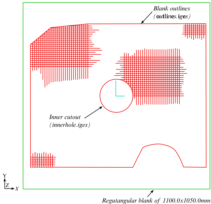
Figure 17-44. A rectangular blank mesh is generated and trimmed into a developed blank shape, with an inner cutout defined by innerhole.iges and outline defined by outlines.iges.
