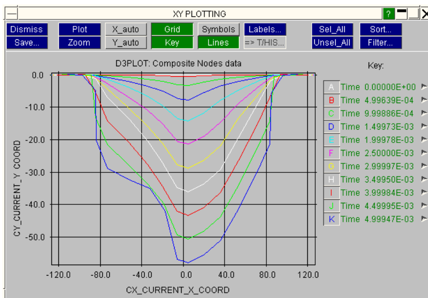
Composite plot of X vs Y coordinates showing formed profile
