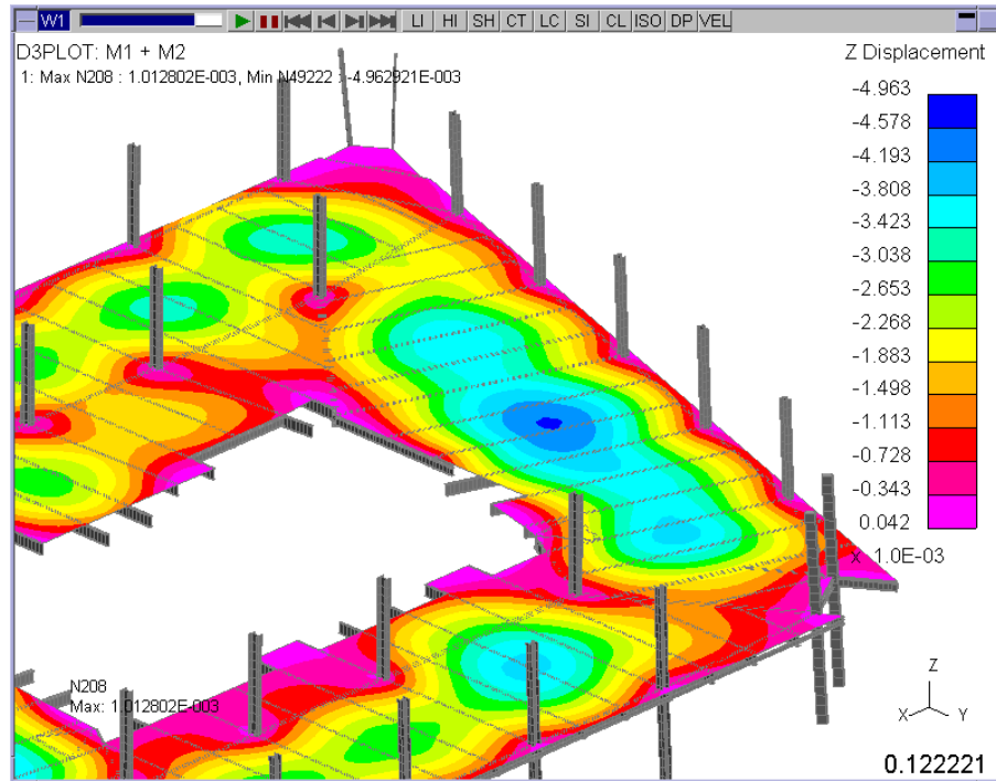
Z Displacement - Beams Excluded
