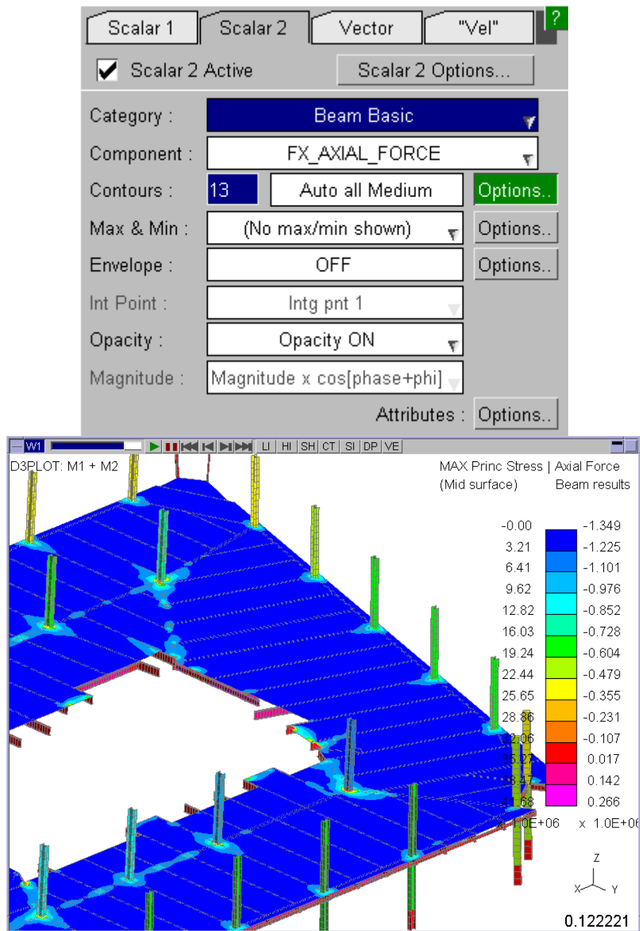
SI plot shows both Max Principal Stress + Beam Axial Force
